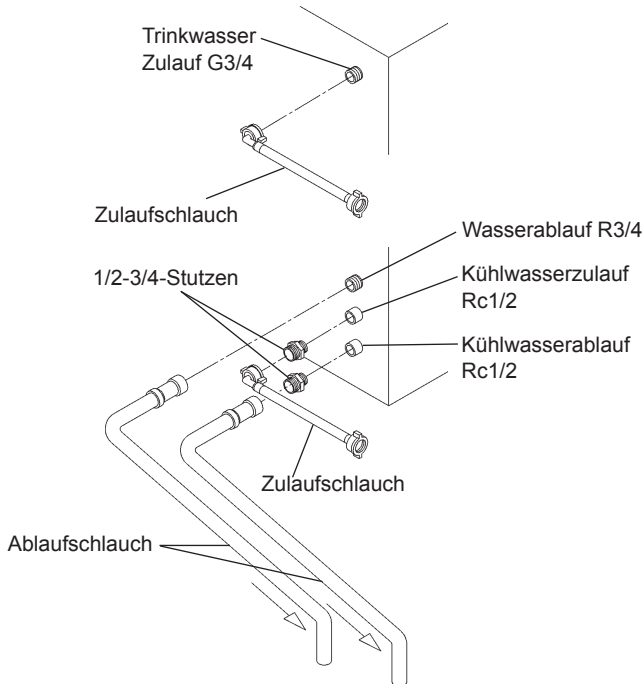
Wassergekühltes Modell [b] (IM-30CWNE/100WNE/130WNE/240WNE)
